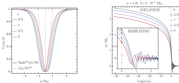
Figure 1: The slow-roll potential from A.A, B.G. and A.S. JHEP 02 (2023) 196.
