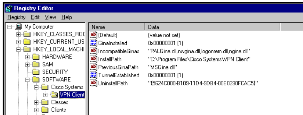
Figure 6-4 Cisco Systems VPN Client Registry Entries
