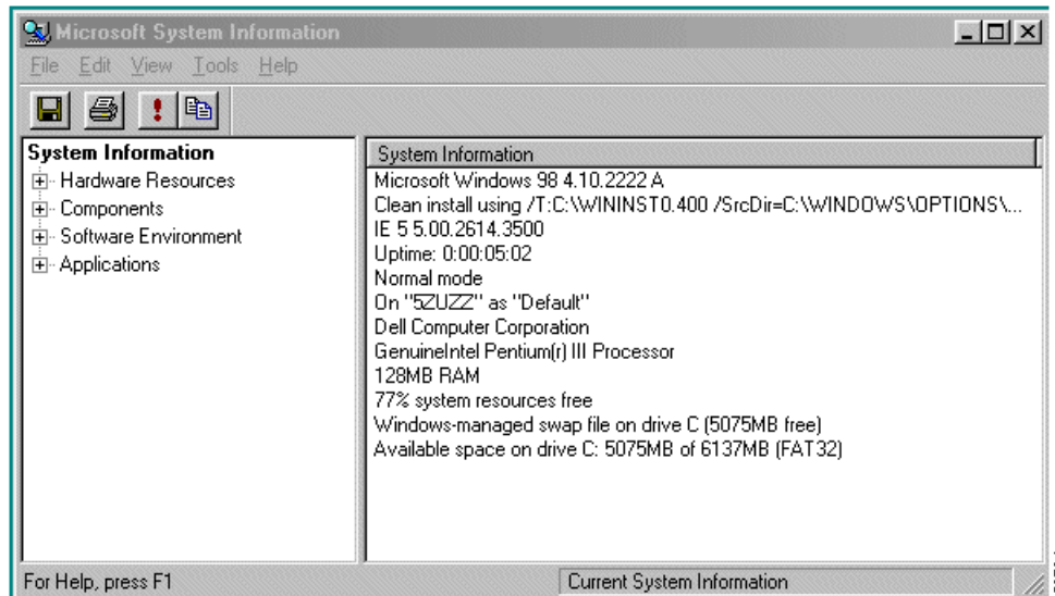
Figure 6-1 System Information Screen on Windows 98
