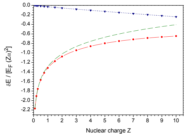
FIG. 2: Numerical and analytical results for the fns correction normalized by the factor of E_F (Z\alpha)^2 , for the 1S state of muonic hydrogen-like ions with the nuclear root-mean-square radius 1 fm, as a function of nuclear charge Z . Solid line and dots (red) represent numerical results (54); dashed line (green) shows analytical results (48); dotted line and triangles (blue) show the difference.
