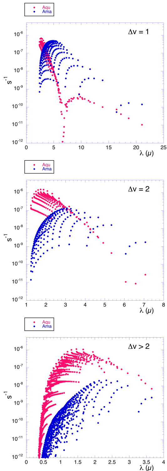
Fig. 1. Electric quadrupole A_{qu} (red) and magnetic dipole A_{ma} (blue) contributions to the transition probabilities in s^{-1} for the Q branches of the H_2 ro-vibrational spectrum within the ground state for \Delta v = 1 , \Delta v = 2 , \Delta v > 2 .
